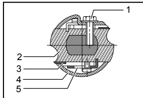
1. Bolt 2. Drum 3. Planer blade 4. Drum cover 5. Adjusting plate
